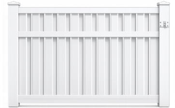
Vertical Shadowbox with Presidential Strips H 36" Thru 72" W 72"
